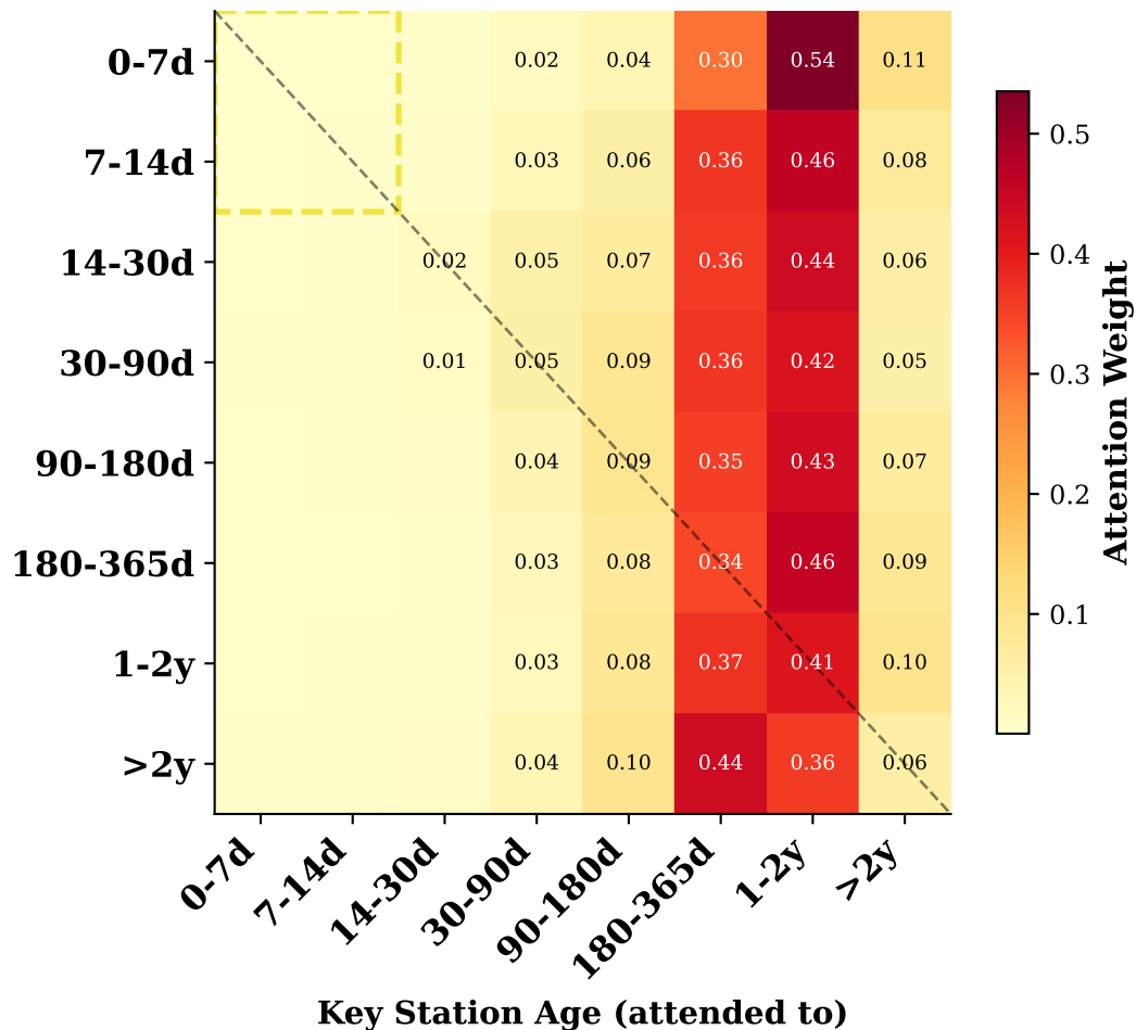
Query Station Age (attending)
